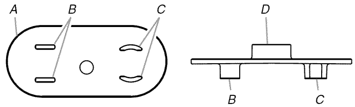
A. Plastic handle spacer B. Straight handle mounting posts
