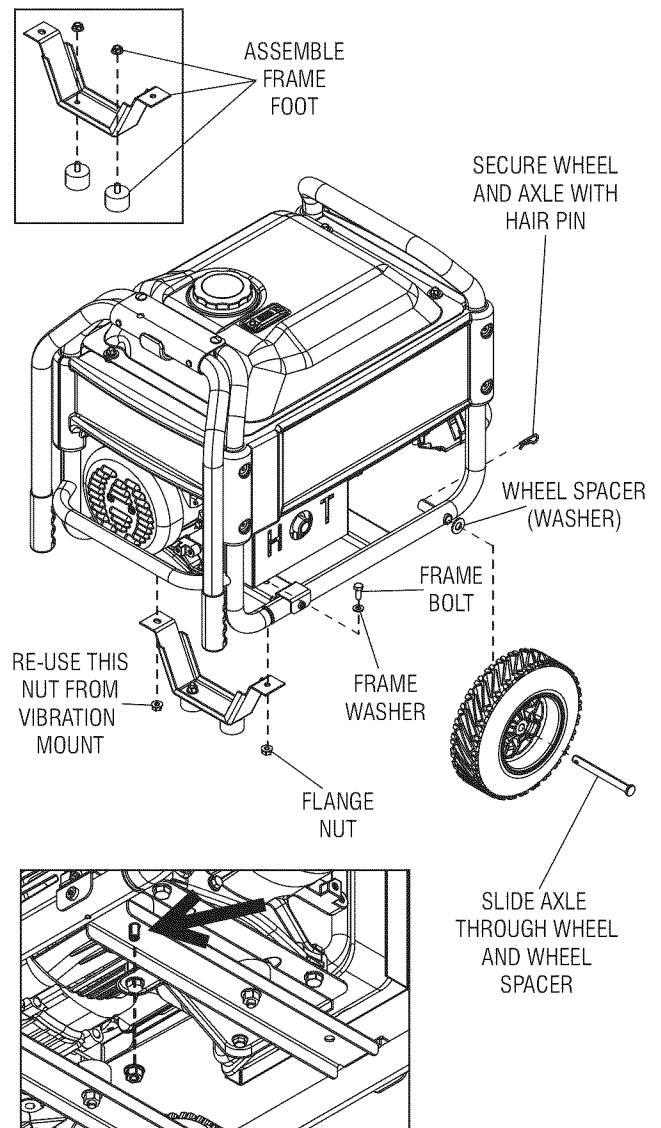
Figure 2 – Wheel and Foot Assembly
