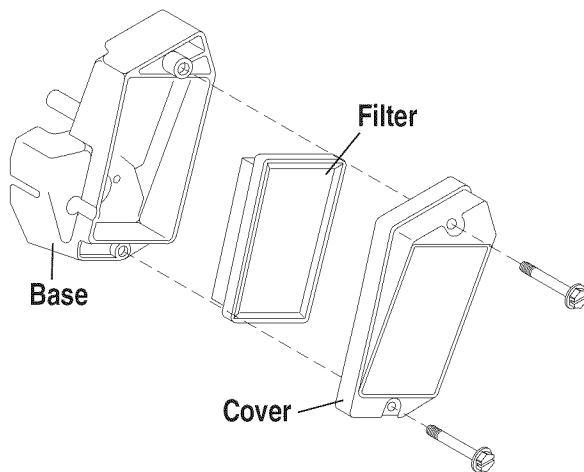
Figure 13 – Air Filter
