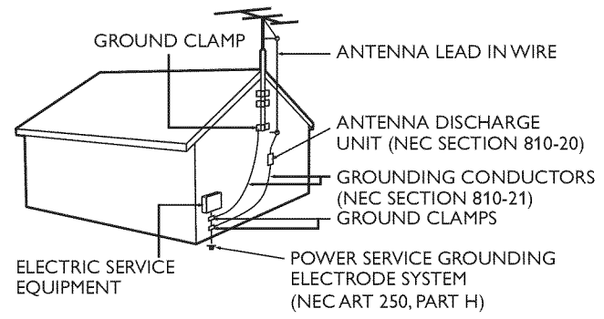
Example of Antenna Grounding as per NEC – National Electric Code
