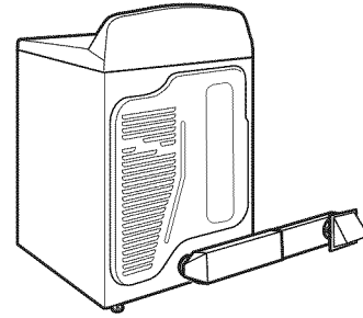
Periscope installation
