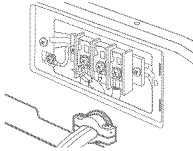
Connecting Electric Dryers (Electric Dryer Type)
