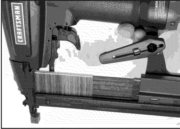
Figure 6—Loading Staples
