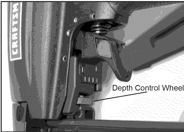
Figure 9-Setting Depth Control
