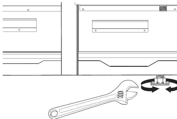
Figure 29: Leveling Legs
