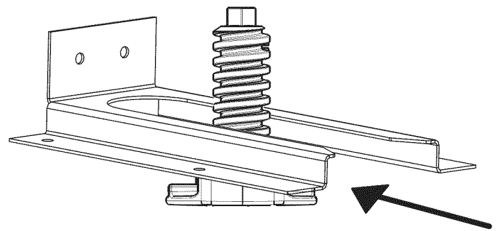
Figure 9: Anti-Tip Bracket
