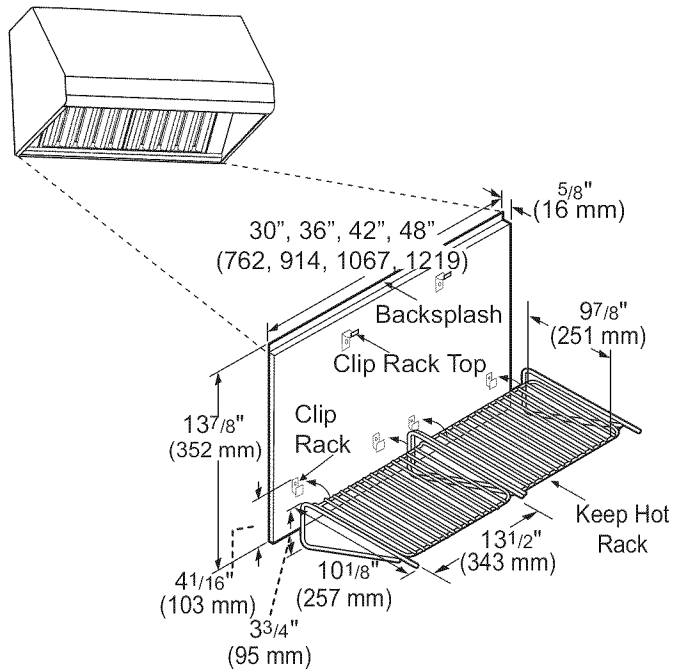
Figure 18: Keep Hot Shelf
