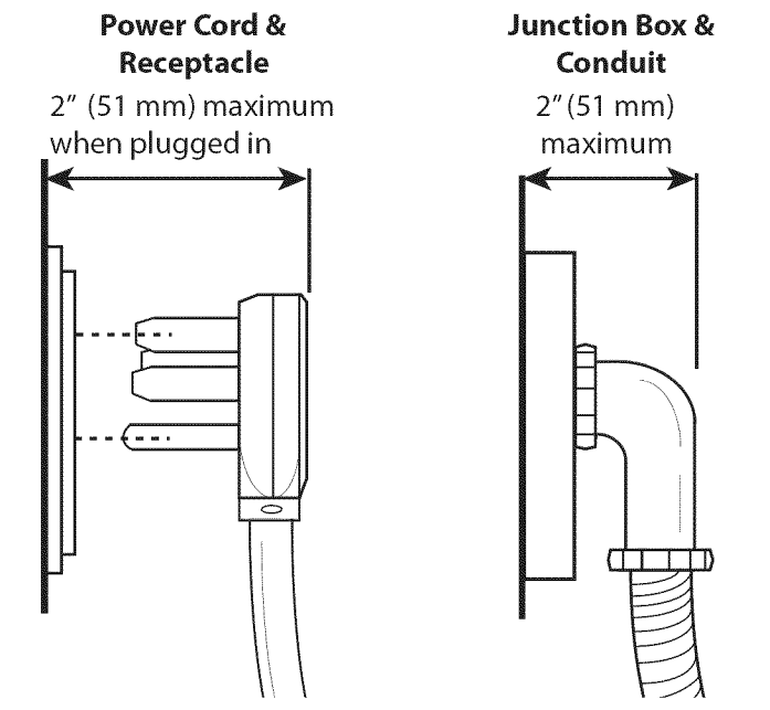
Figure 5: Wall Connection
