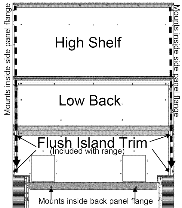
Figure 22: Backguard Installation
