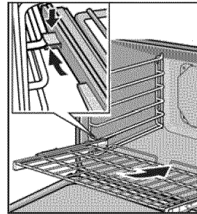
Figure 2: Full Access Oven Rack
