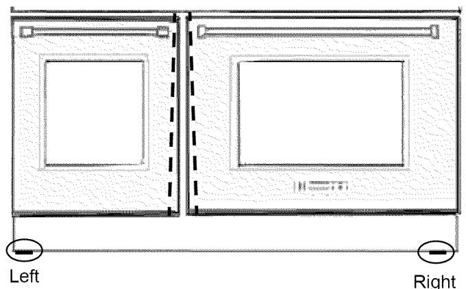
FIGURE 10: 48" DOOR ALIGNMENT
