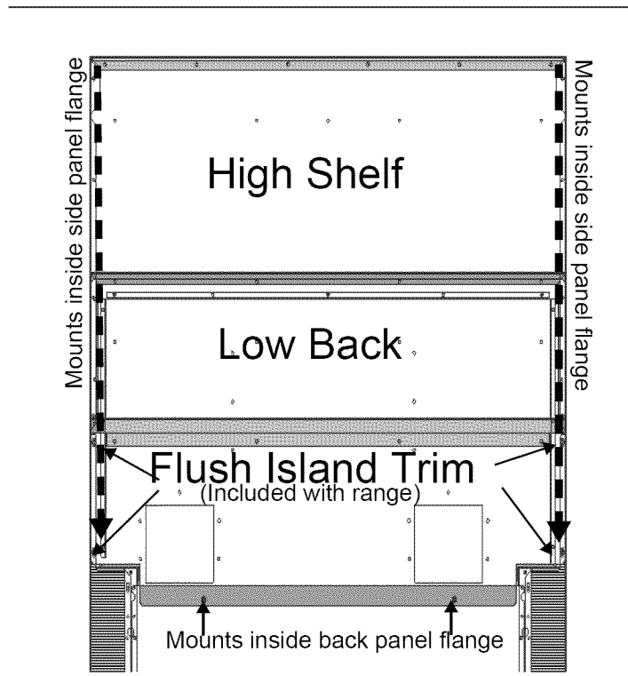
FIGURE 21: BACKGUARD INSTALLATION
