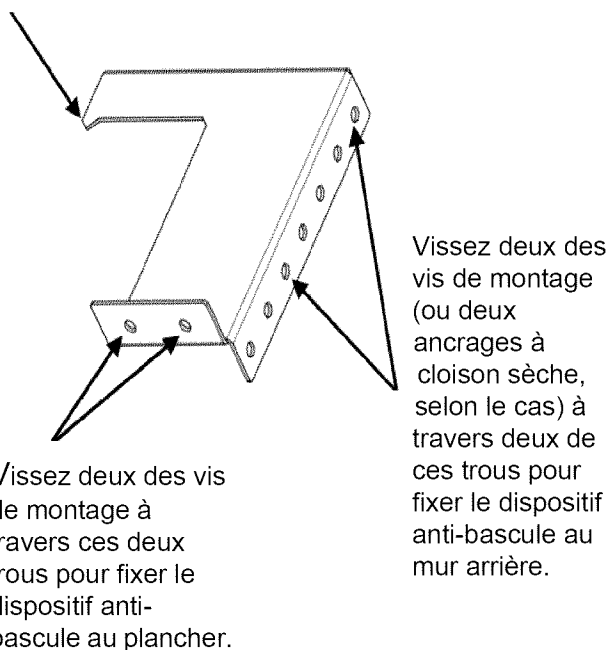
FIGURE 11: SUPPORT ANTI-BASCULE
