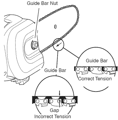
Figure 6 - Saw Chain Adjustment
