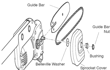
Figure 1 - Installing Guide Bar
