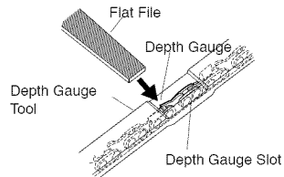
Figure 16 - Depth Gauge Tool On Chain
