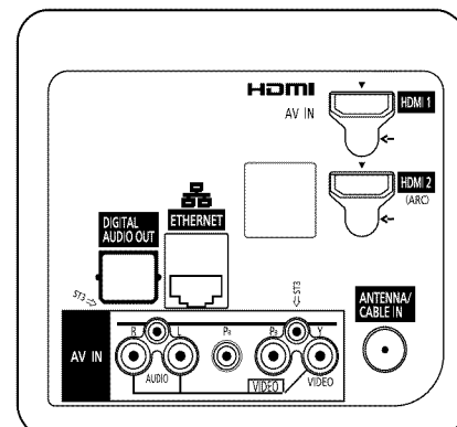
Rear Panel
