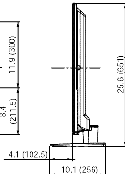
Side view with the pedestal (option) attached
