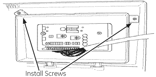
Install Screws
