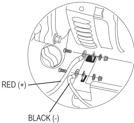
Figure 15 - Battery Connections
