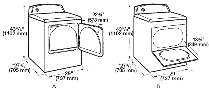
A. Wide opening side-swing door B. Wide opening hamper door
