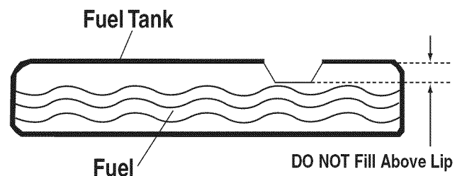
Figure 9 - Fuel Tank
