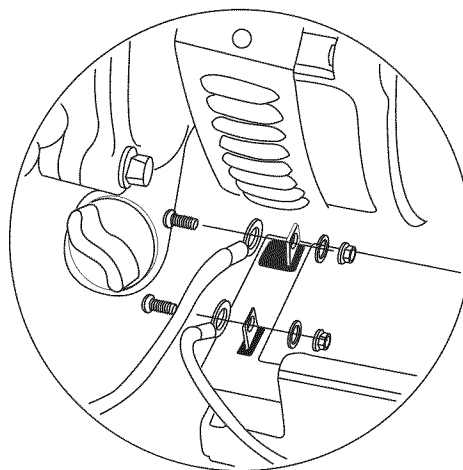
Figure 15 - Battery Connections
