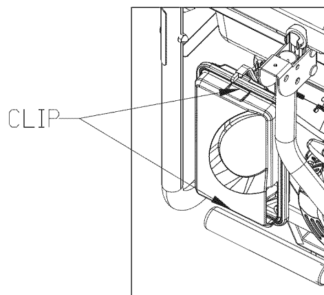
Figure 16 - Air Filter
