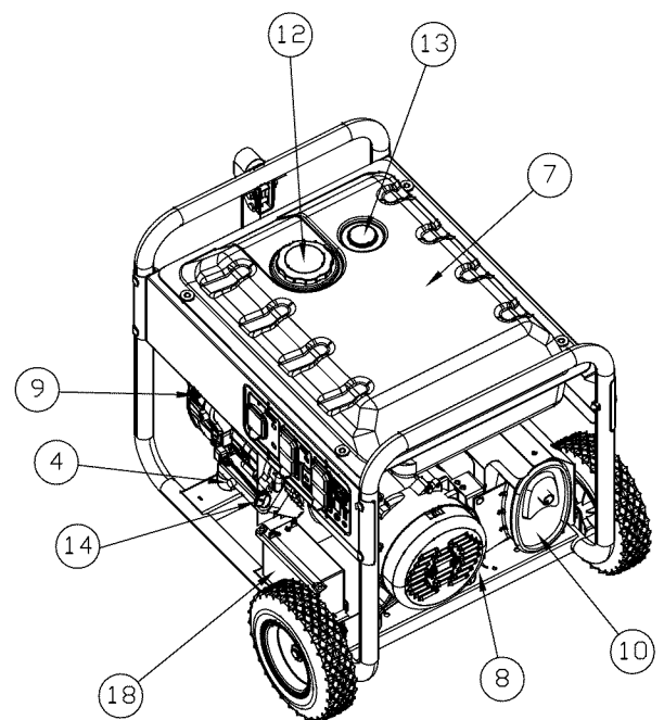
Figure 4 - Generator Controls
