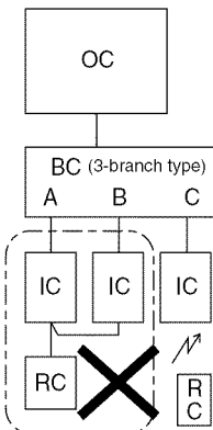
3-1. Group operation by single remote controller
