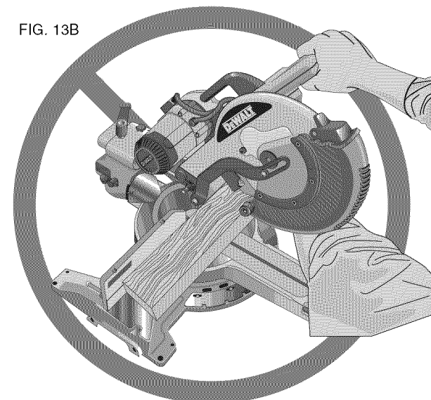
IMPROPER CUT
