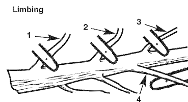
Cut Limbs One at a Time and Leave Support Limbs Under the Tree Until the Log is Cut
