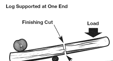
First Cut - 1/3 Diameter
