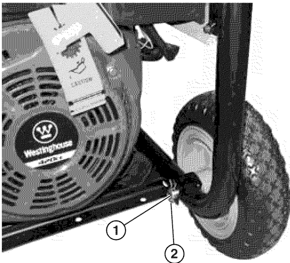
Figure 13 – Assemble Wheels to Frame
