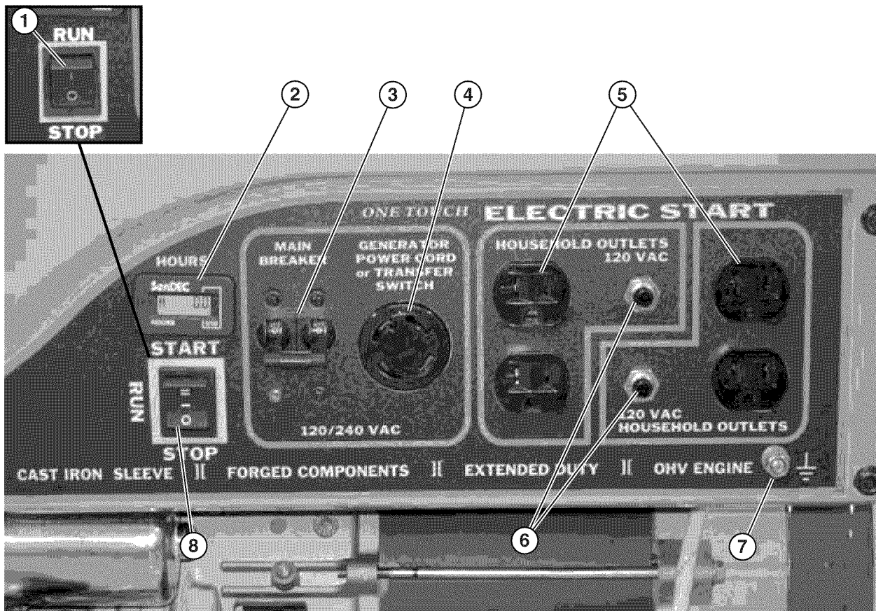
Figure 18 – Control Panel Features
