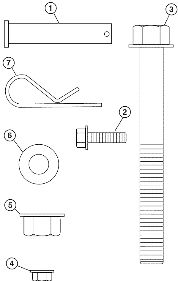
Figure 3 – Wheel Kit Hardware for Serial Number XXXXXX0612 and Earlier
