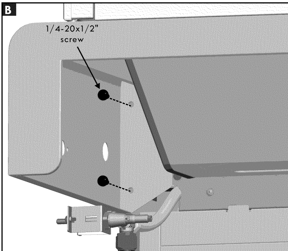
1/4-20x1/2" Screw Qty. 2
