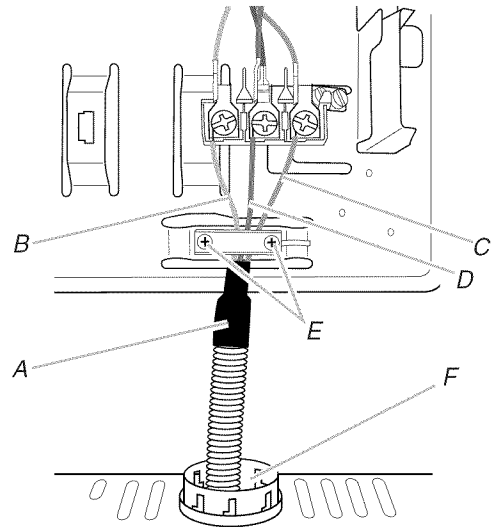
A. CSA approved flexible conduit B. Black wire (L1) C. Yellow/green wire (GND) D. Red wire (L2) E. Screws F. Opening in oven bottom
