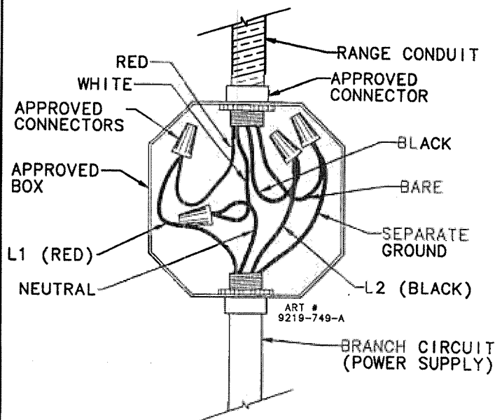
WIRING METHOD IF CODE DOES NOT PERMIT GROUNDING THROUGH NEUTRAL CONDUCTOR & ALSO REQUIRED IN MOBILE HOMES.
