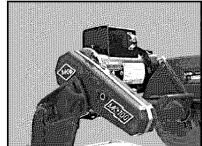
(C) Install the Cutting Head onto the Post Pivot Shaft and install the Adjusting Knob.
