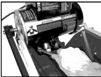
(G) Loosen the two front motor mounting bolts. If re-tension- ing only, go to step N.
