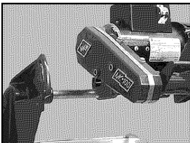
(G) Install the Cutting Head in rear Pivot Hole (Cutting Head Adjustment pg 25).
