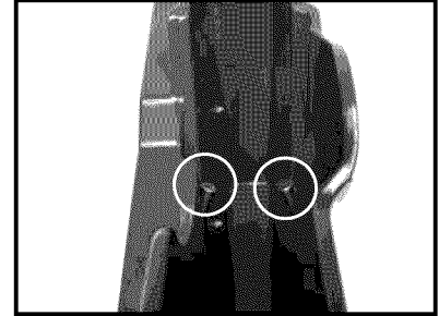
(C) Run the MK-100 until clear water is seen at the blade cooling ports (Approx. 1 min.)
