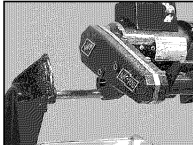
(B) Align Cutting Head Rear Pivot Hole to the Post Pivot Shaft and slide onto shaft.
