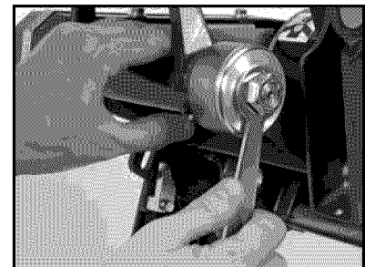
(C) Depress and hold the Shaft Lock button and remove Retaining Nut and Outer Flange using the Blade Wrench.
