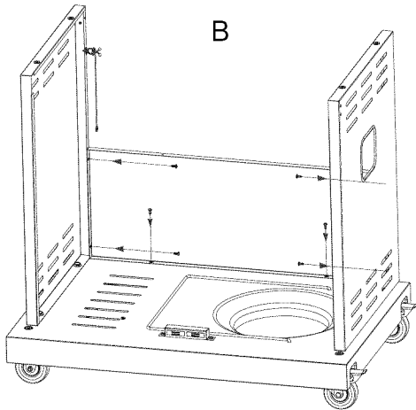
M4X10 screws Qty: 16 pcs
