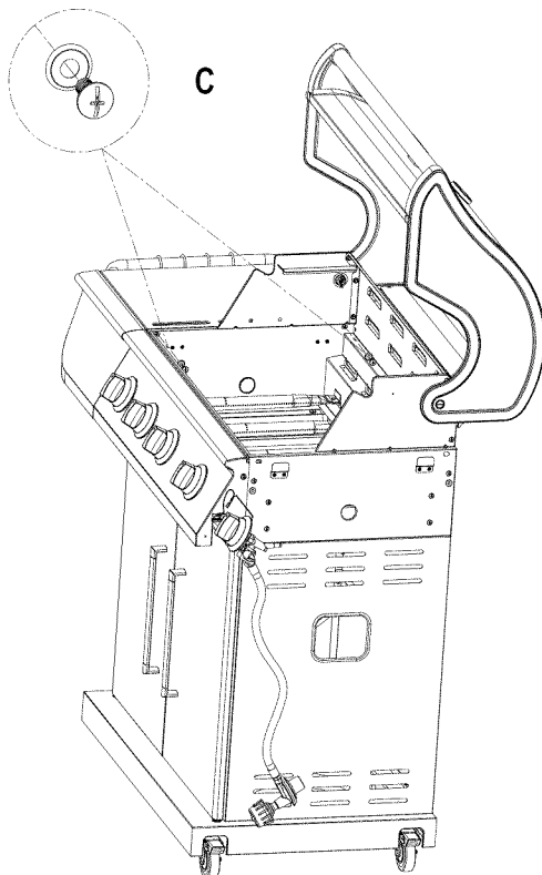
M6 compression washer Qty: 2 pcs
