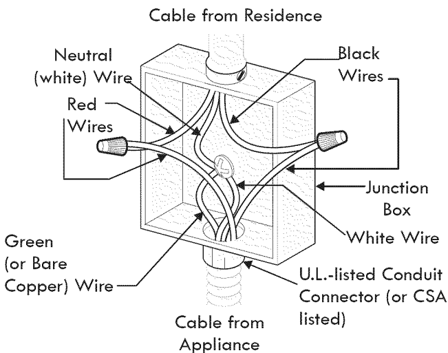
Figure 10 3-Wire (Grounded Neutral) Electrical System (Example: Junction Box)
