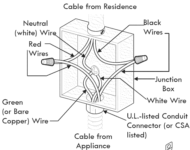
Figure 11 4-Wire Electrical System (Example: Junction Box)
