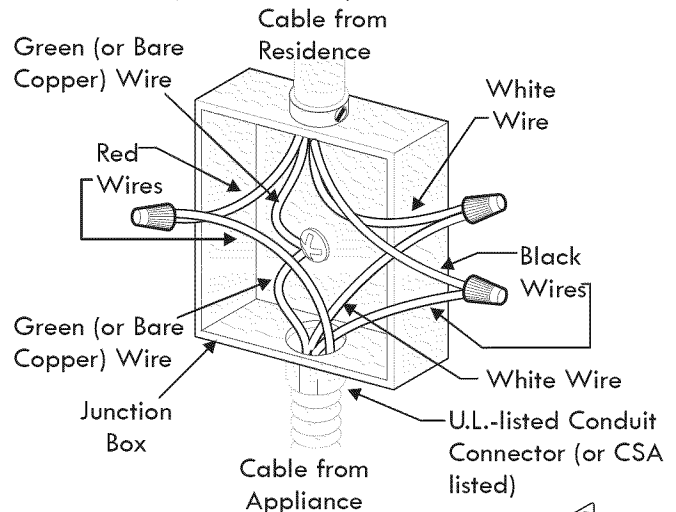
Figure 11 4-Wire Electrical System (Example: Junction Box)
