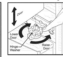
Raising/Lowering Door
