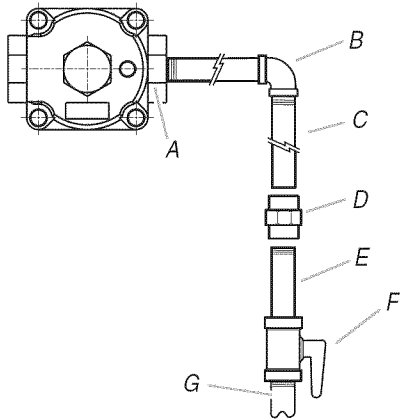
A. Pressure regulator connection fitting B. 90° elbow C. Black iron pipe D. Union E. Nipple F. Manual shutoff valve G. 1/2" or 3/4" gas pipe
