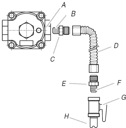
A. Pressure regulator connection fitting B. Use pipe-joint compound. C. Adapter D. Flexible connector E. Adapter F. Use pipe-joint compound. G. Manual shutoff valve H. 1/2" or 3/4" gas pipe
