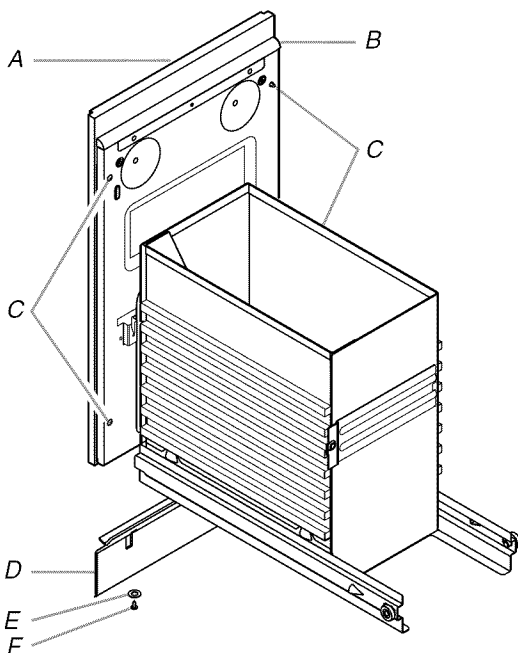
A. Custom panel B. 15" (38.1 cm) x 1/2" (13 cm) quarter-round C. Panel screw locations D. Toe guard E. Washer F. Toe guard mounting screw
