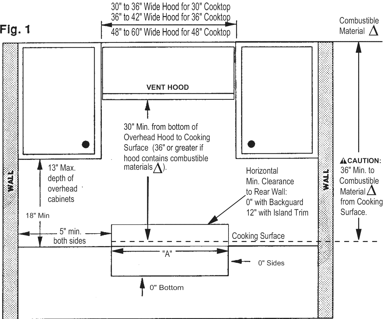
Figure 1: Clearance Requirements
