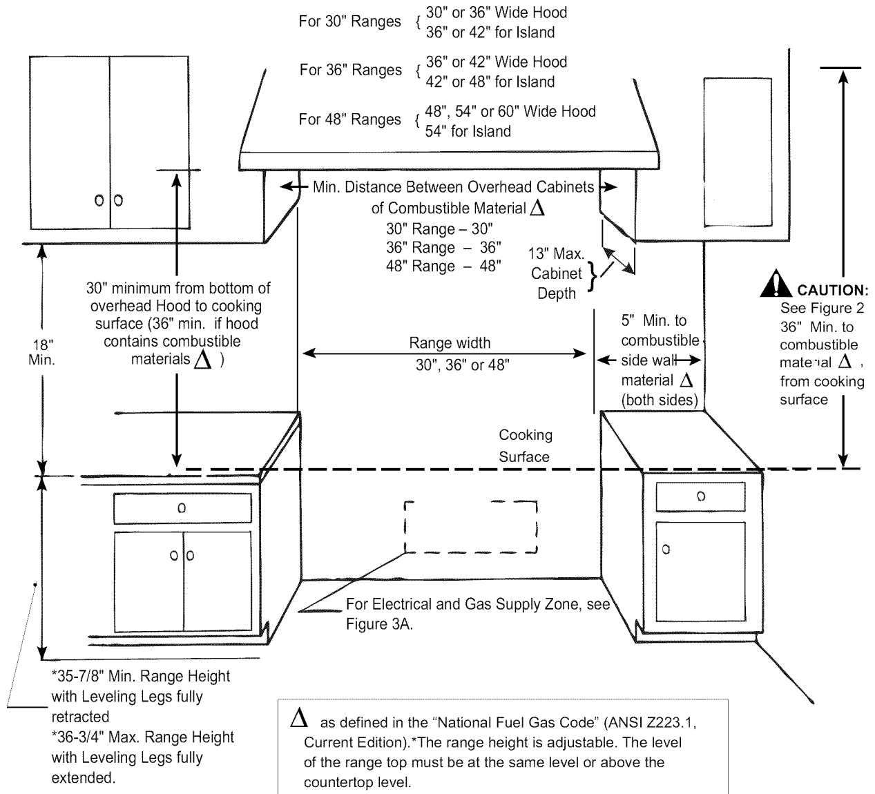
Figure 1: Cabinet Clearances
