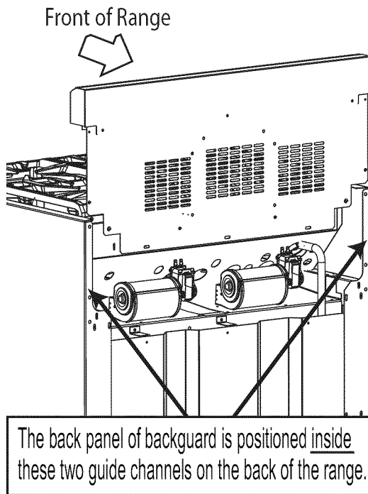
Figure 16: Backguard Positioning
