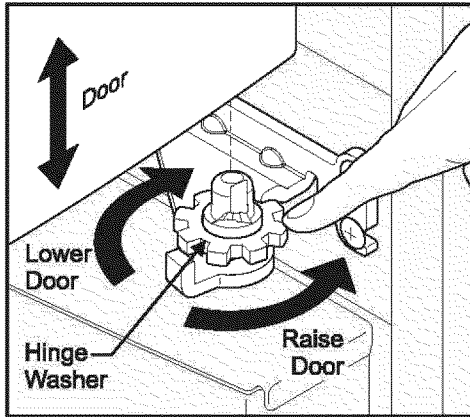
Raising/Lowering Door
