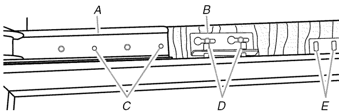
A. Top hinge B. Panel top bracket C. Holes for screws D. Door adjustment pins E. Holes for screws (36" Models only)
