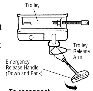
Lockout position (Manual disconnect)
