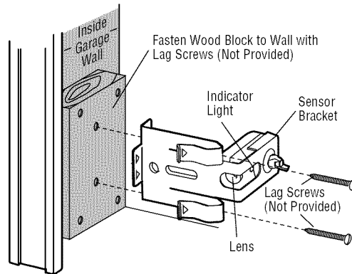
Figure 3 WALL MOUNT (RIGHT SIDE)
