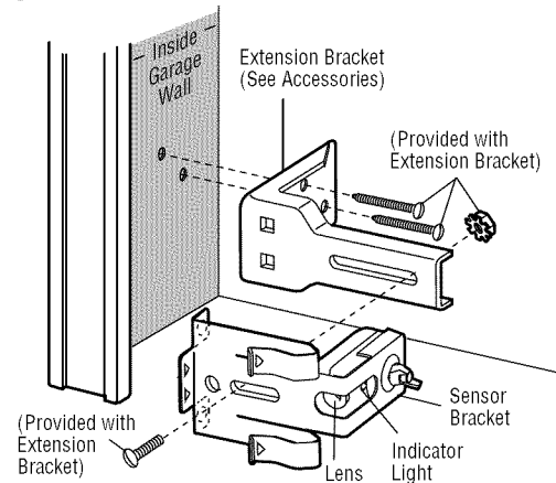
Figure 3 WALL MOUNT (RIGHT SIDE)
