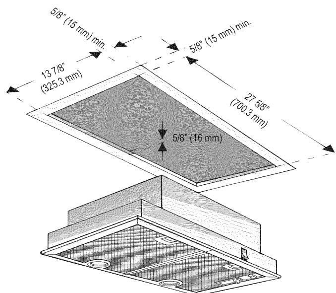
Figure 8: Housing Cutout Dimensions - 28 3/4" (73 cm) models
