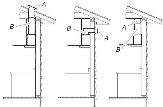
A. Roof cap B. 8" (20.3 cm) round vent
