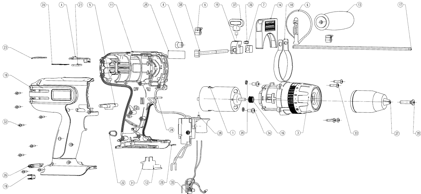
20.0 VOLT LITHIUM-ION CORDLESS 1/2-in. HAMMER DRILL / DRIVER MODEL NUMBER 320.29004
