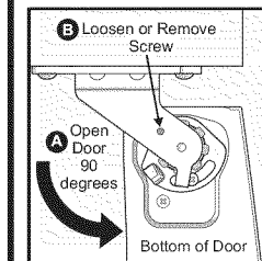
Remove Screw
