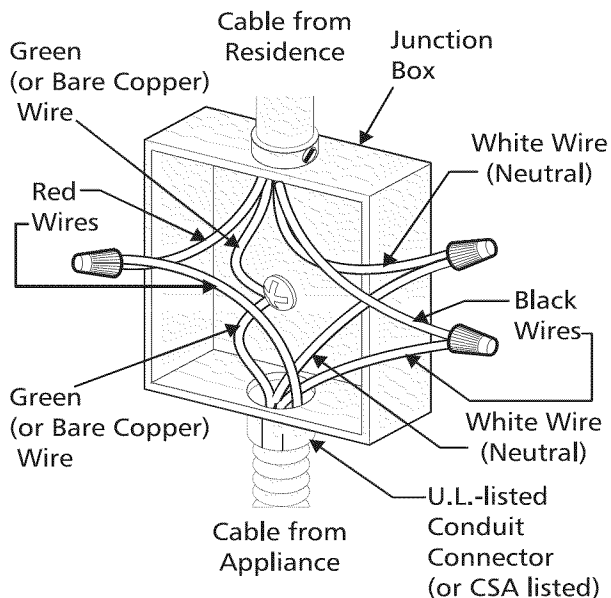
Figure 8 – 4-Wire Electrical System (Example: Junction Box)
