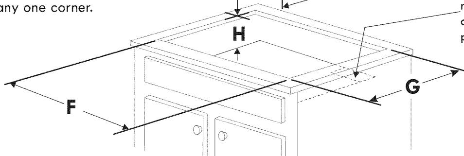
Cooktop Cutout Dimensions
