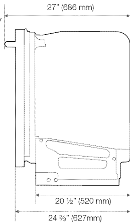
Side view (DMT800 series/ DMT400 series)
