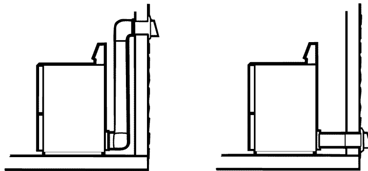
Correct Venting
