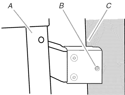
A. Door front facing B. Side bracket screw hole for cabinet attachment C. Cabinet front
