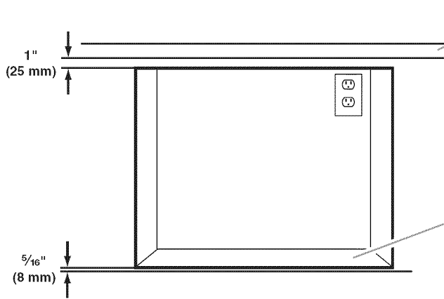
A. Cutout floor B. Cabinet, storage drawer, oven or warming drawer
