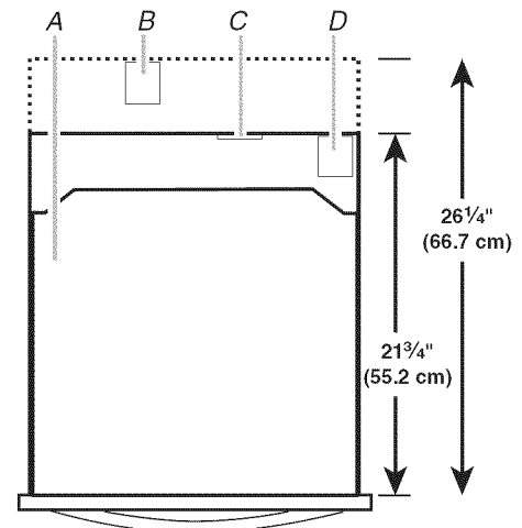
A. Microwave oven B. Non-flush receptacle C. Flush receptacle D. Non-flush receptacle located in upper right or upper left corner
