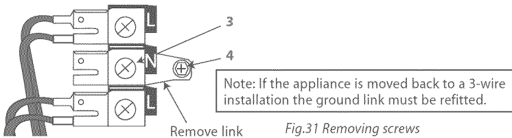
Fig.31 Removing screws
