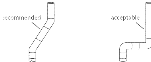
Fig.12 Duct configurations
