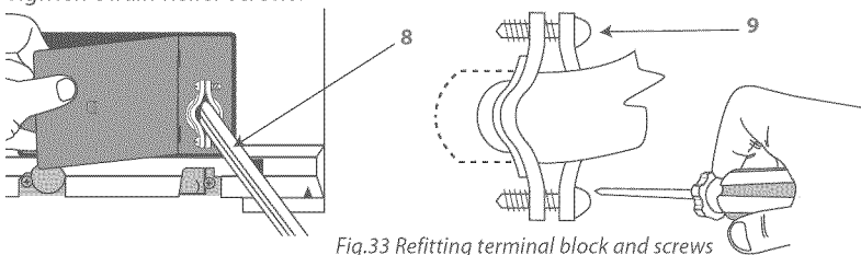
Fig.33 Refitting terminal block and screws
