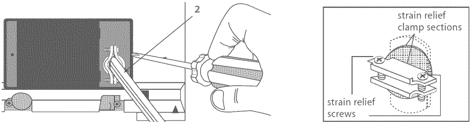
Fig.30 Inserting the power cord
