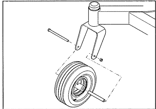
Caster wheel
