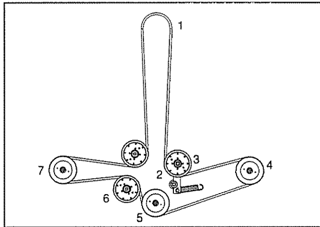
Belt routing, deck belt
