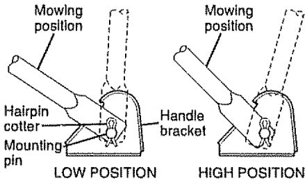
LOW POSITION
