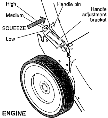
HIGH POSITION
