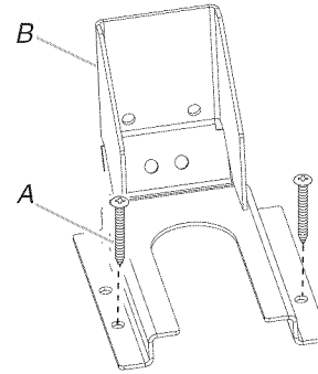
A. #12 x 1 \frac{1}{8} " screws B. Anti-tip bracket
