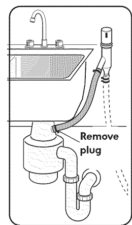
To a disposer dishwasher drain connection through an air gap.
