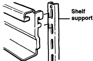
Make sure both sets of hooks are in support slots.
